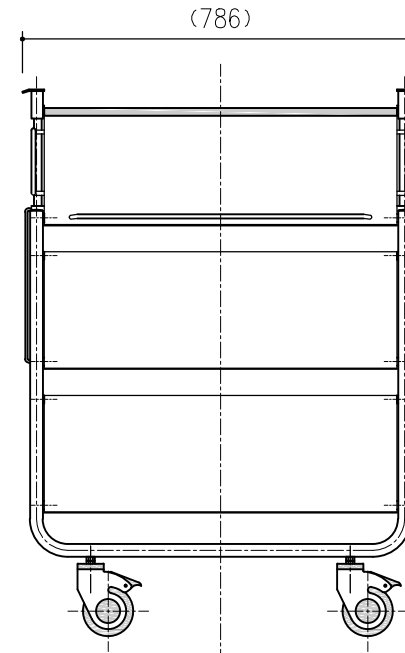
Smart_Wagon_Upper_Fold_3PT
