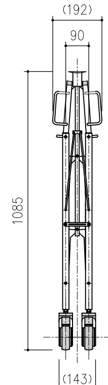
Smart_Wagon_Side_Fold_3PT
